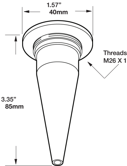
Beam Cone 100.703.5
