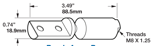
Break-Away Bar
