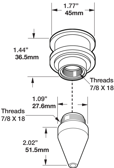
Adapter Tip 100.703.3 5mm
