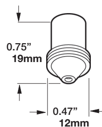
Nozzle, Outer 216-20722 .080
