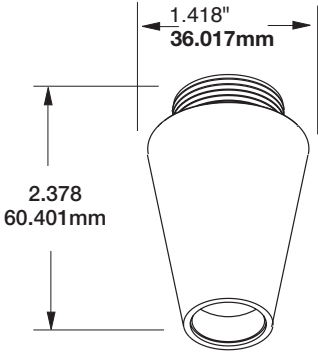
Sensor Head 71341622
