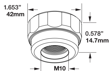
Nozzle Body Threaded
