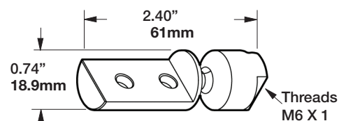
Break-Away Bar
