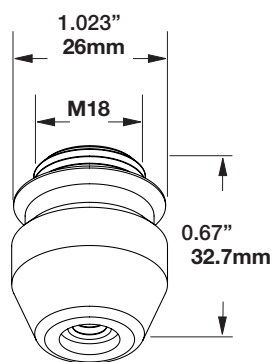
Nozzle Holder
