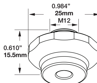
Nozzle EAC
