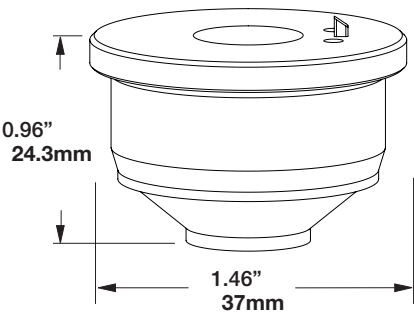
Nozzle Holder ceramic HCH-S01201
