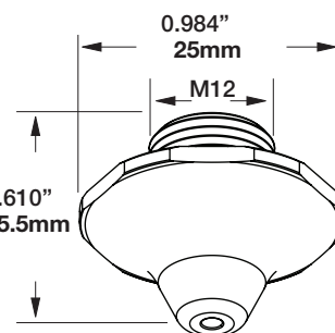
Nozzle EAB
