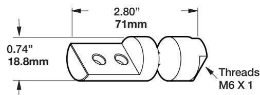
Break-Away Bar
