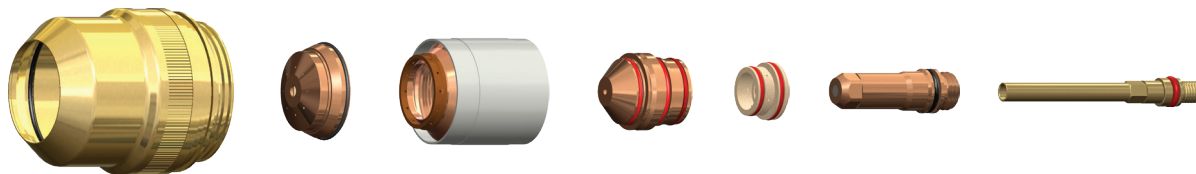
260 amp Stainless Steel consumables illustrated above
