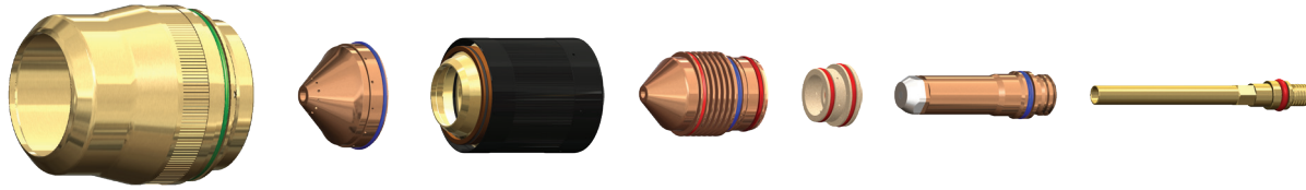
260 amp Mild Steel consumables illustrated above
